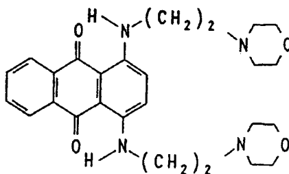
Compound 1d
